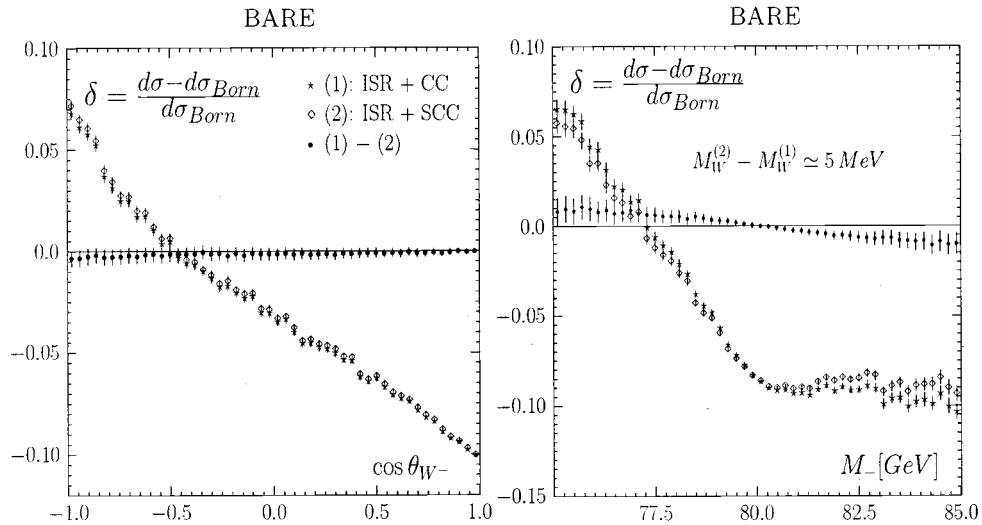
FIG. 2. Effects of the screened Coulomb correction (SCC) on the distributions of the polar angle (left) and the invariant mass (right) of W^- in comparison with the usual Coulomb correction (CC) at E_{c.m.} = 200 GeV. As indicated the star, solid diamond, and large dotted curves are the ISR+usual Coulomb correction, ISR+screened Coulomb correction, and their difference respectively, in the presence of YFS exponentiation. Results are for the e^+e^- \rightarrow W^+W^- \rightarrow u\bar{d}\mu^-\bar{\nu}_\mu channel. The bare cut is that of Sec. 4.1 of Ref. [11].
