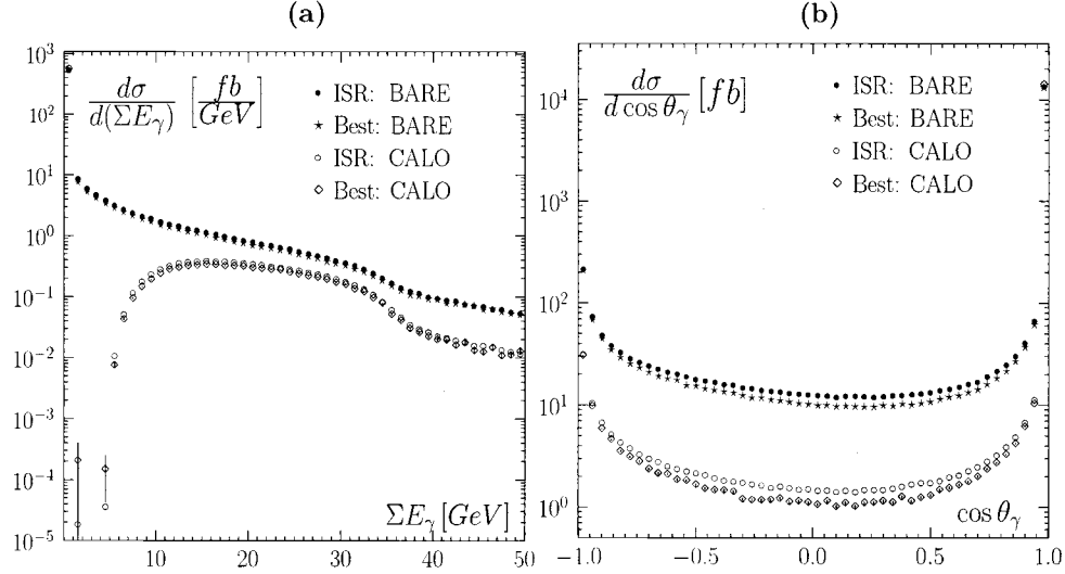
FIG. 1. Distributions of the total photon energy (a) and cosine of the hardest photon polar angle (b) for the u\bar{d} + \mu^+\bar{\nu}_\mu + n(\gamma) final state. The solid, open circle, star, and diamond curves correspond to the LL BARE, LL CALO, \mathcal{O}(\alpha)_{\text{prod}} \mathcal{O}(\alpha^2) LL FSR BARE, and CALO YFS-exponentiated results, respectively.
